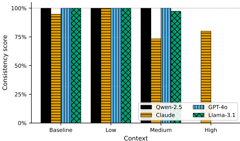
ESPR — Cross-run Consistency by Vagueness Level
